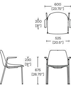
OLA/1/A Four Leg Arm
