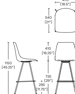
OLA/7 Four Leg Barstool (Plastic Shell)
