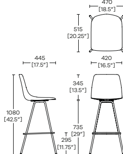
OLA/7 Four Leg Barstool (Wood Shell)
