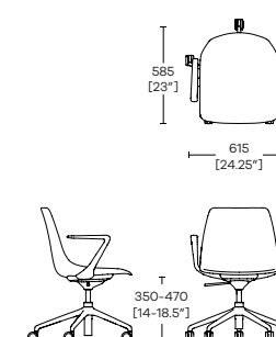
OLA/5/ZA 5 Star Tilt Armchair (Only available fully uph or with seat pad)
