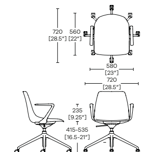
OLA/4/HA/ZA Low 4 Star Tilt Armchair (Only available fully uph or with uph seat pad)
