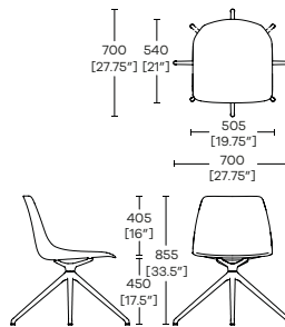
OLA/4 High 4 star with spider
