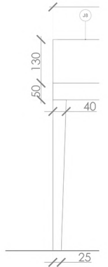
3 BEDSIDE TABLE SIDE ELEVATION SCALE 1:5
