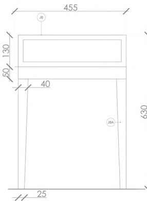
2 BEDSIDE TABLE FRONT ELEVATION SCALE 1:5
